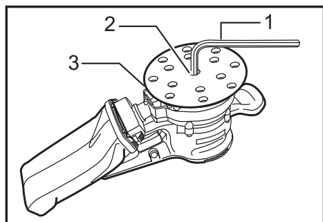
► 1. Hex wrench 2. Screw 3. Pad
